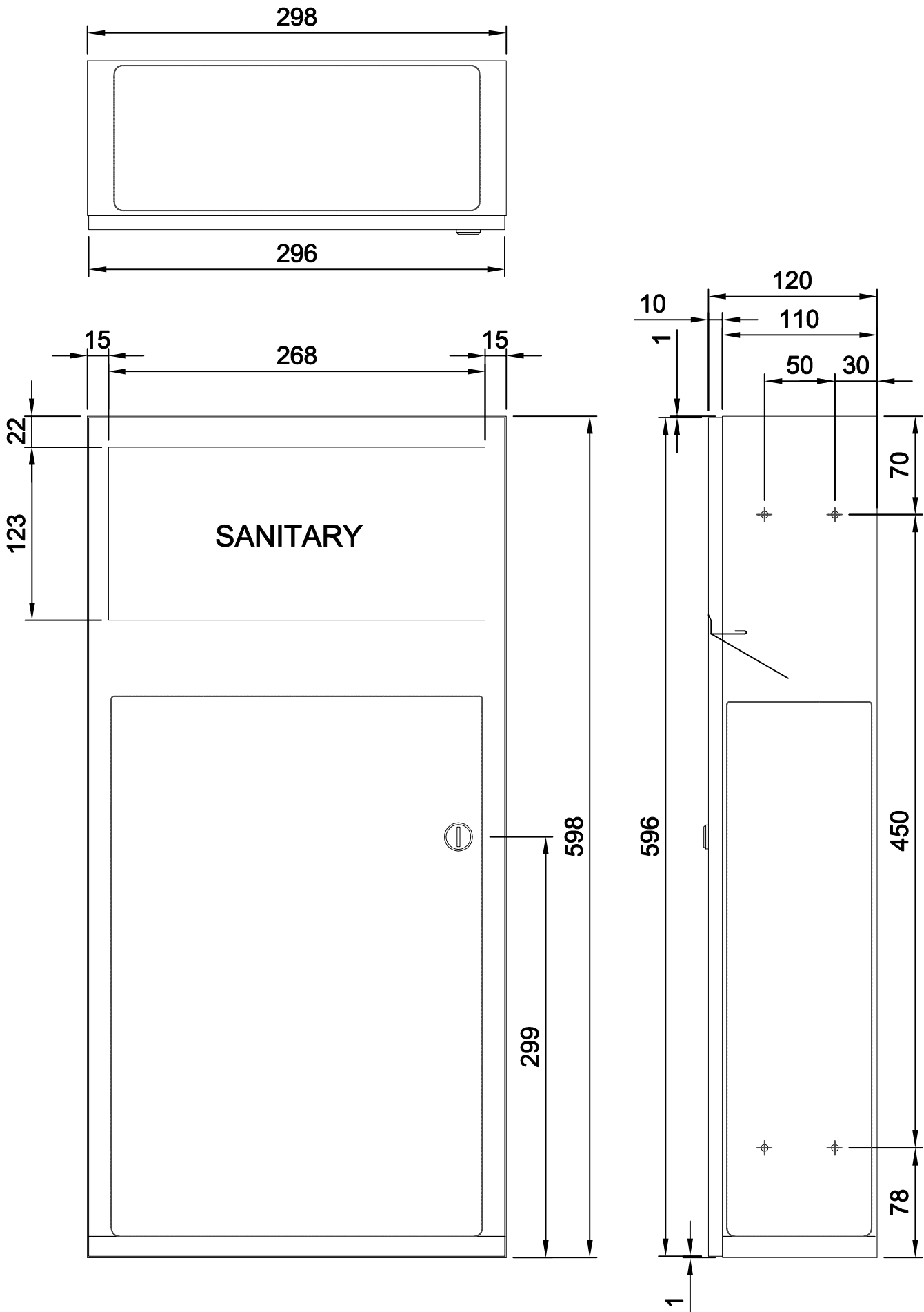
DOLPHIN SOLUTIONS LIMITED DOLPHIN RECESSED SANITARY WASTE BIN WITH FLAP DP5110-SAN
